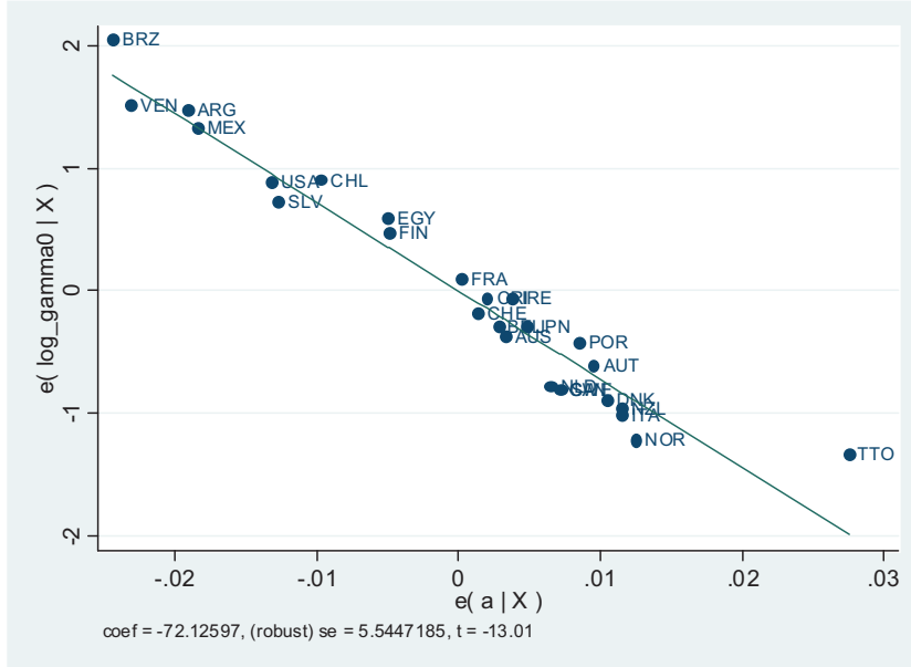
Figure 6: The Strehler-Mildvan Correlation
