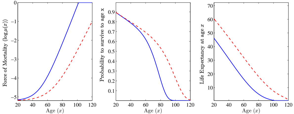
Figure 5: Aging Before and After the Wonka-Vite
