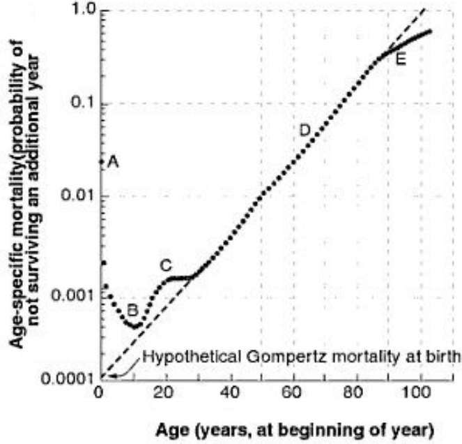
Figure 1: Age-specific Mortality Rate: United States 1959-1961
