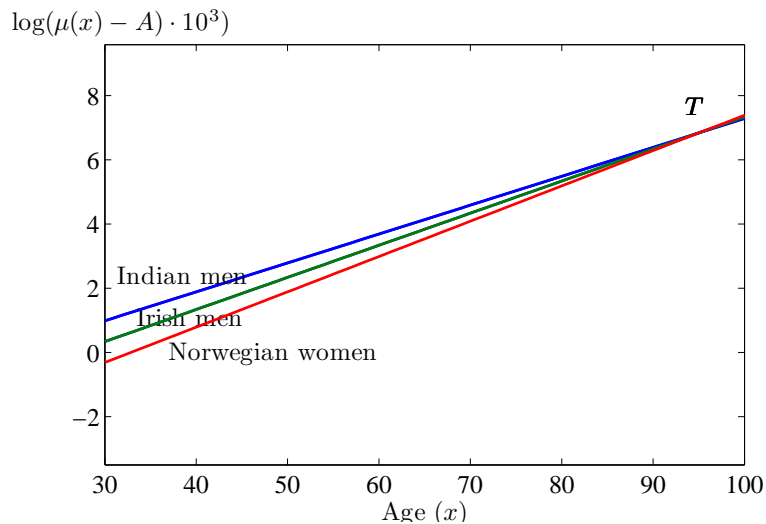
Figure 7: The Strehler-Mildvan Correlation
