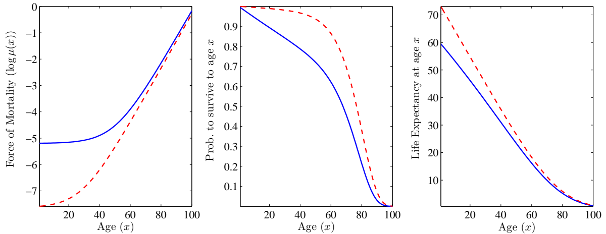
Figure 3: Aging In Sweden 1901-1910 and 1983
