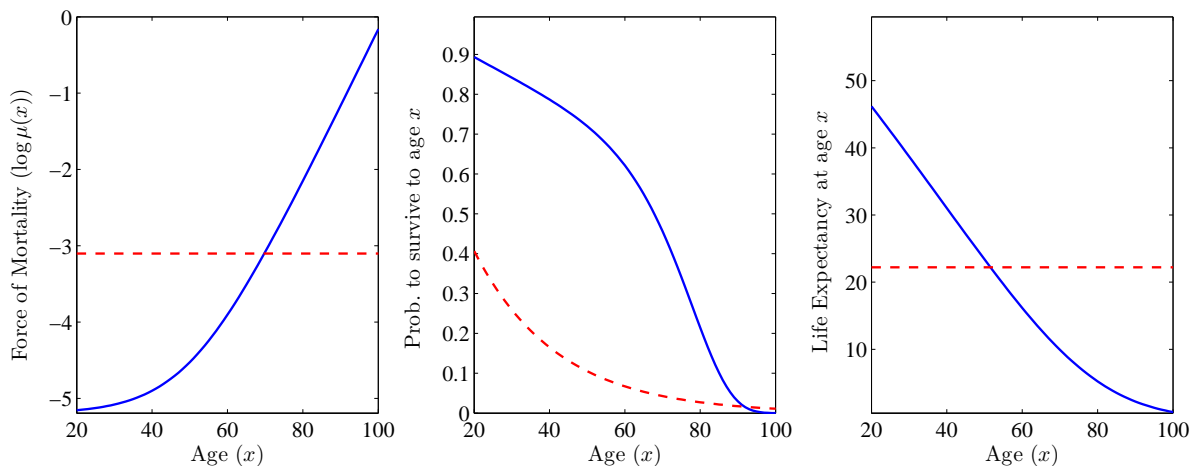
Figure 2: Aging according to Gompertz-Makeham vs. Probabilistic Death
