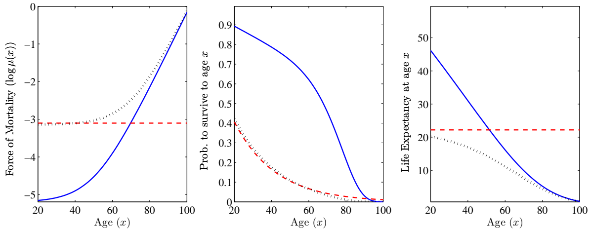
Solid lines: Estimates from Swedish life tables as in Figure 2. Dashed lines: hypothetical perpetual youth scenario: \lambda = 0.025 as in Figure 2. Dotted lines: Gompertz-Makeham with elevated background risk A = 0.43 .
